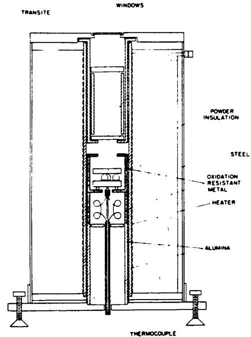
FIG. 5 Typical Furnace
