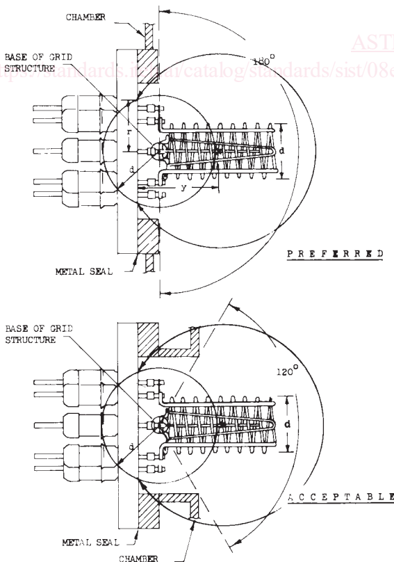
FIG. 2 Flange-Mounted Nude Ionization Gage
