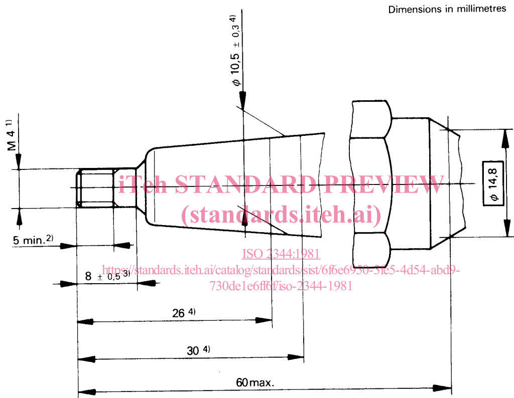
Figure 4 – Threaded terminal
