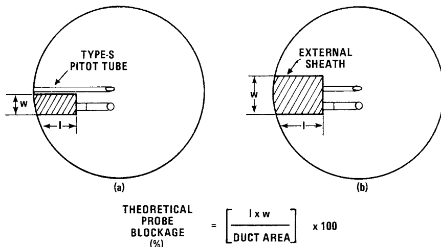
FIG. 5 Projected-Area Models for Typical Pitobe Assemblies
