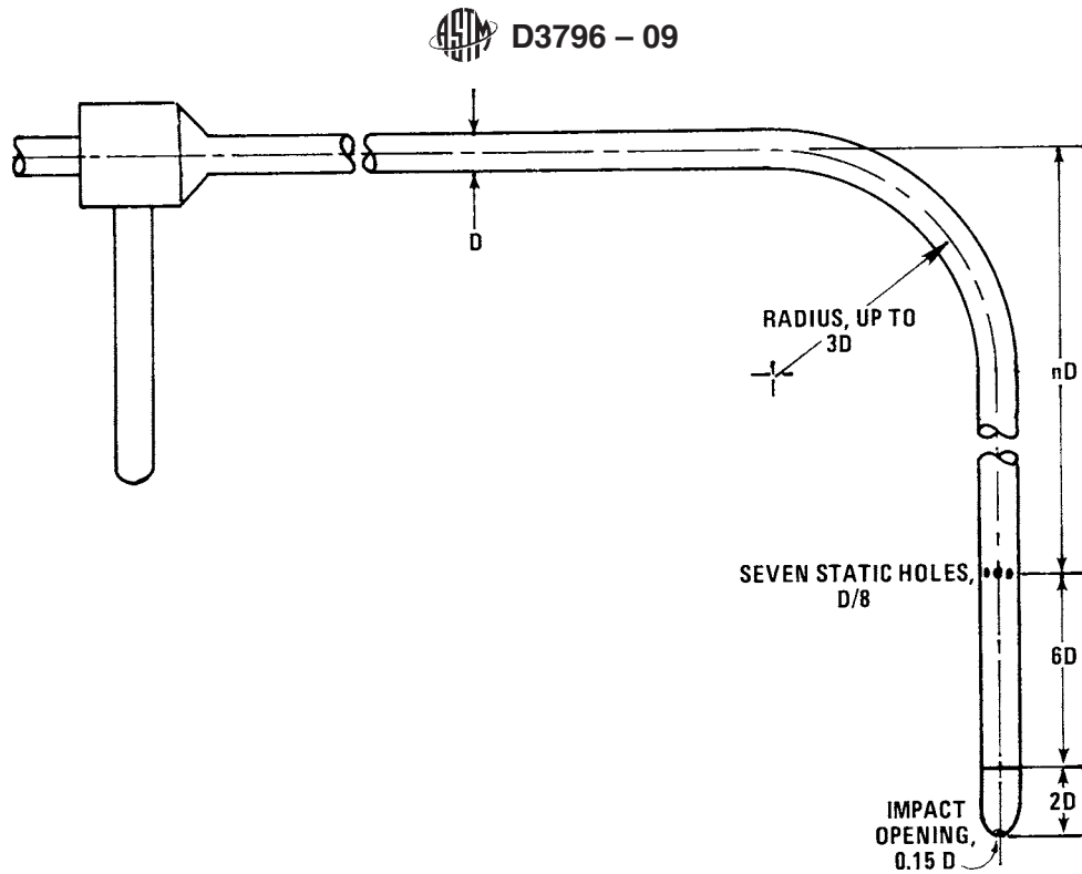
FIG. 3 Ellipsoidal Nosed Pitot-Static Tube
