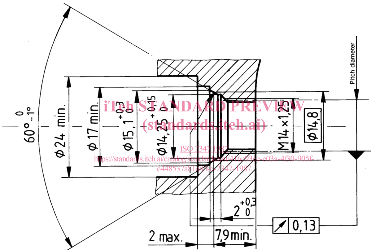
Figure 2 — Housing of the spark-plugs in the cylinder head
