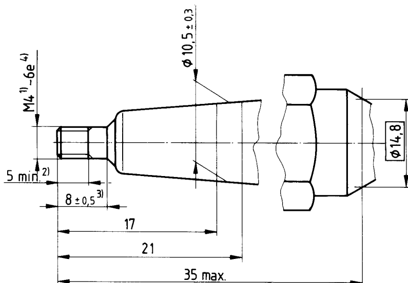
b) threaded terminal
