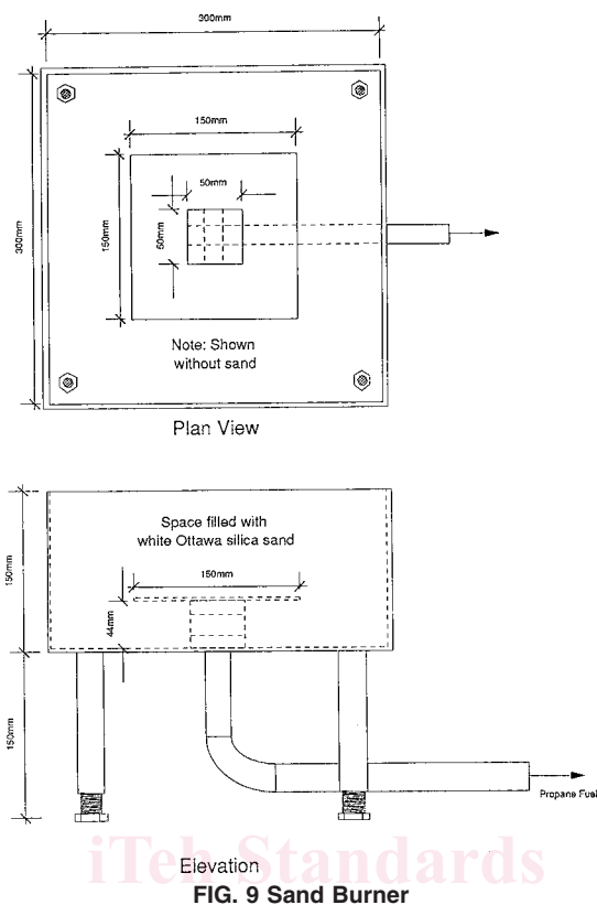
FIG. 9 Sand Burner
