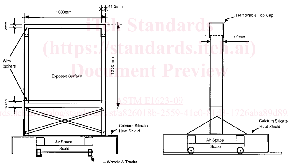
FIG. 2 Sample Holder
