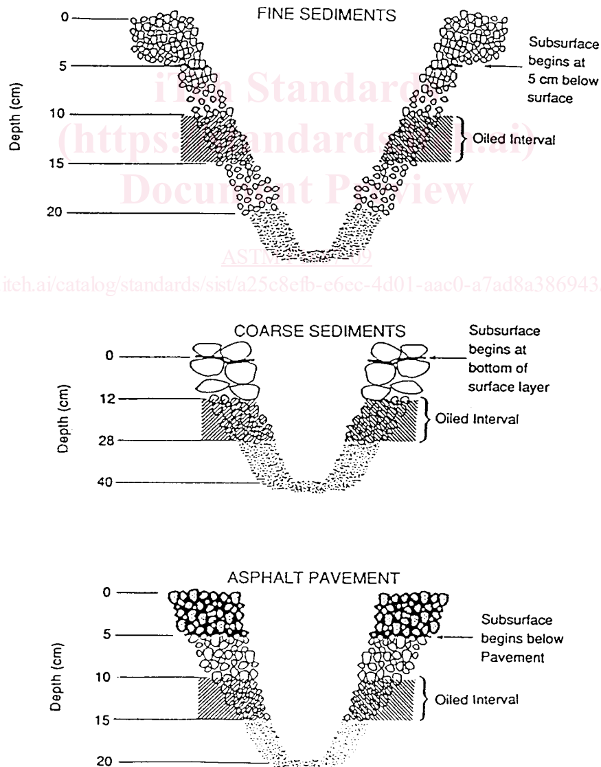
FIG. 1 Subsurface Boundaries for Various Beach Types 53
