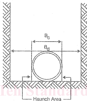
TRENCH CROSS SECTION
