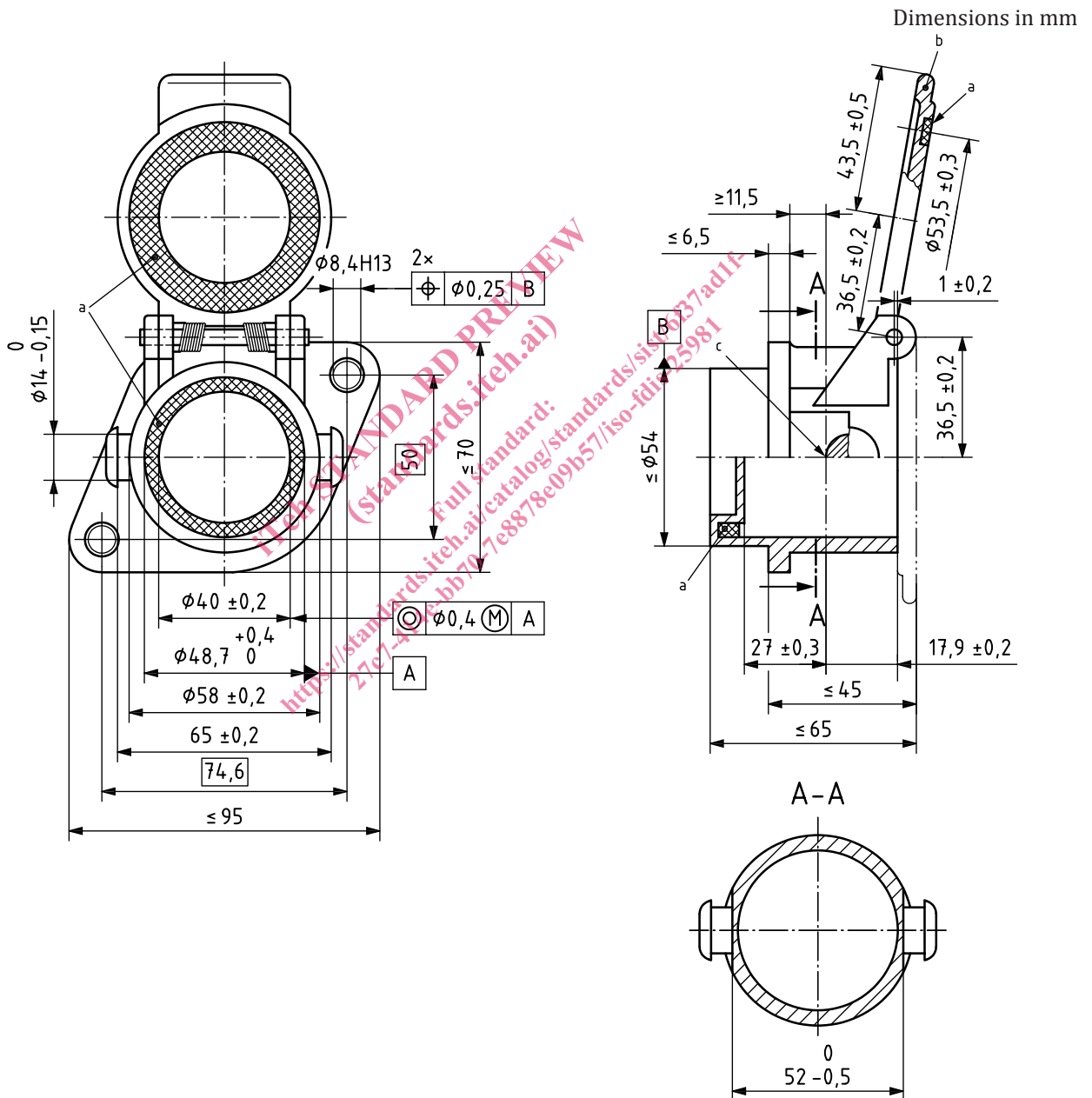
Figure 2 — Socket
