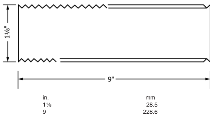
FIG. 3 Metal Test Piece Thin Film Liquid Contact
