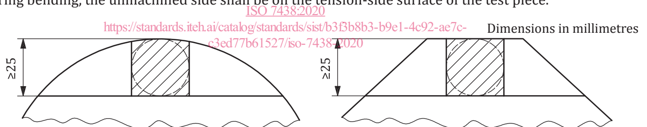
Figure 4 — Diameter and inscribed circle diameter of the test piece
