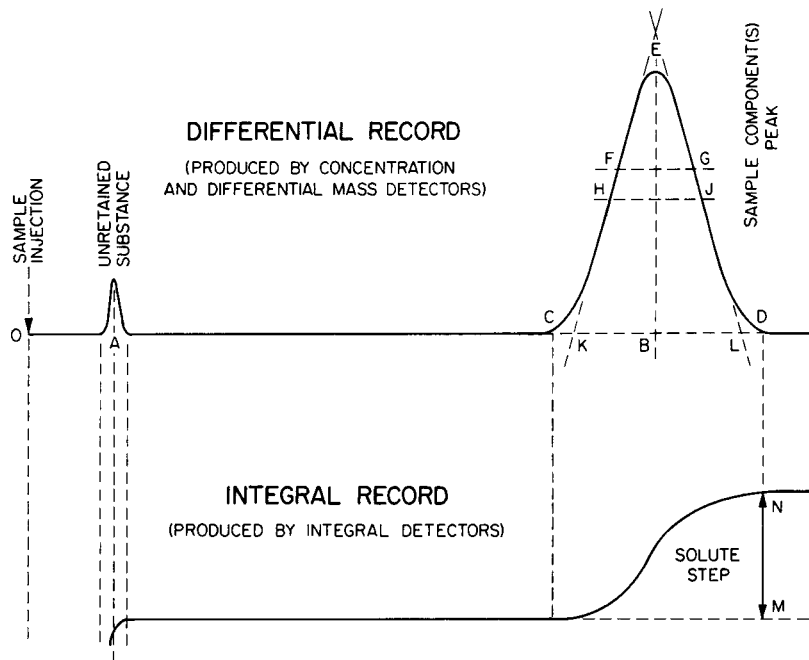
FIG. 1 Typical Chromatogram.
