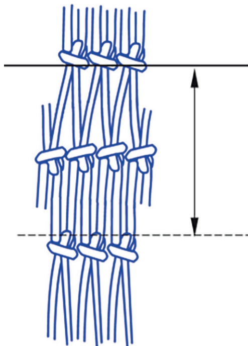
Figure 3 — Measure of mesh opening iTeh STANDARD PREVIEW (standards.iteh.ai)
