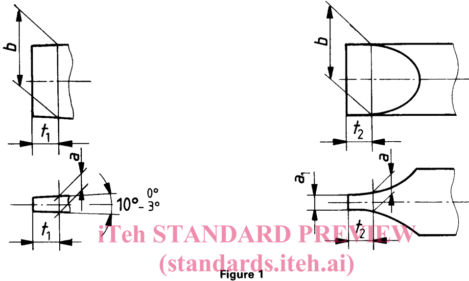
Type B (for hand-operated screwdrivers) Type C (for machine-operated screwdrivers)
