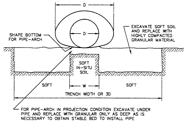
FIG. 4 Soft Foundation Treatment
