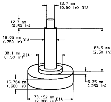
FIG. 1 Core Splice Adhesive Mold
