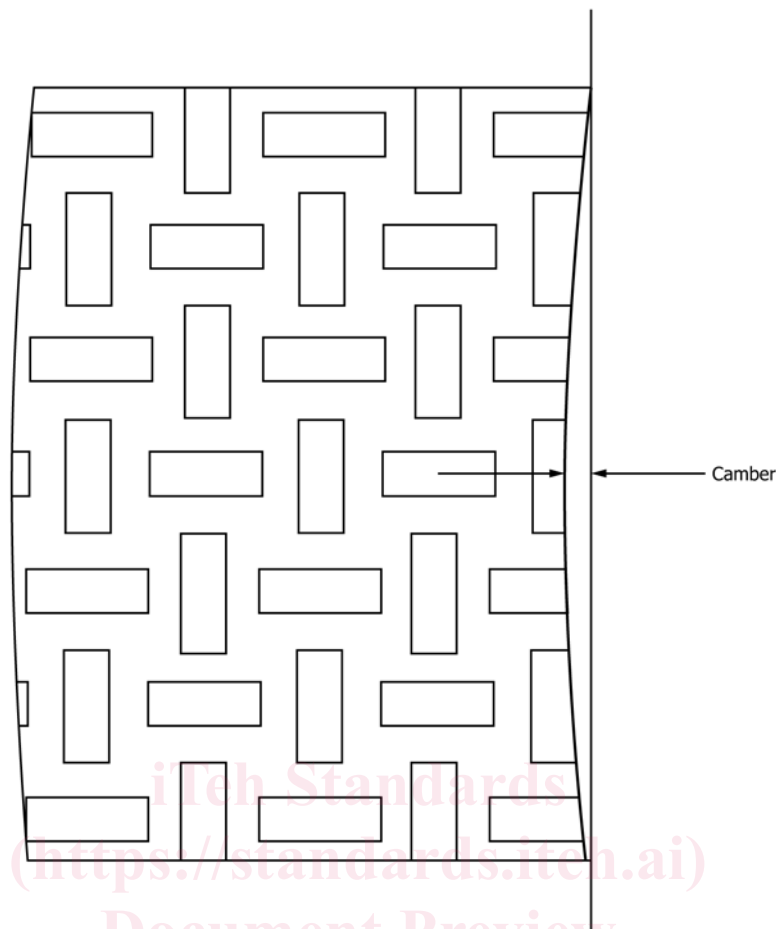
FIG. 4 Camber for Rectangular Sheared Floor Plates and Gas-Cut Floor Plates (see Table 5 or Table A1.4)
