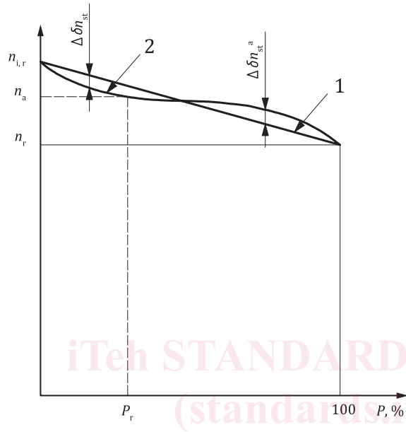
Figure 1 — Speed/power characteristic, range of speed setting
