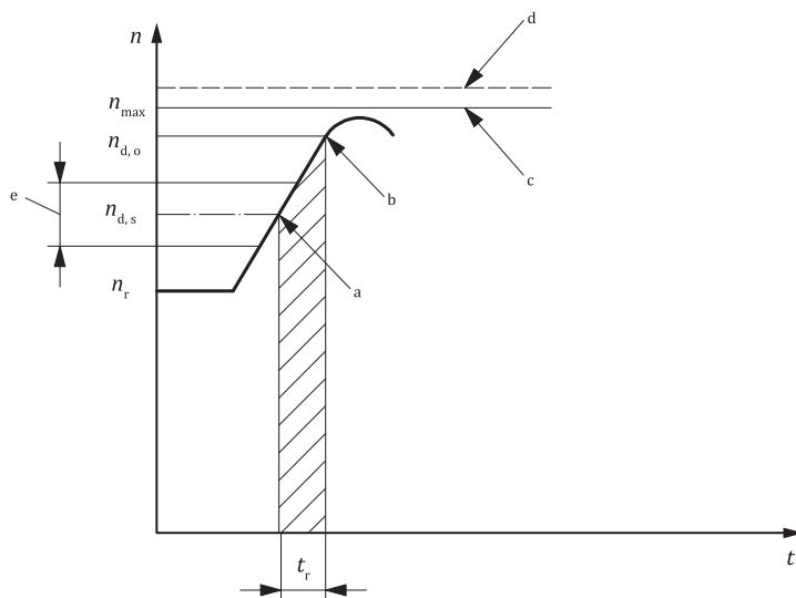
Figure 2 — Speed/power characteristic deviation from the linear curve
