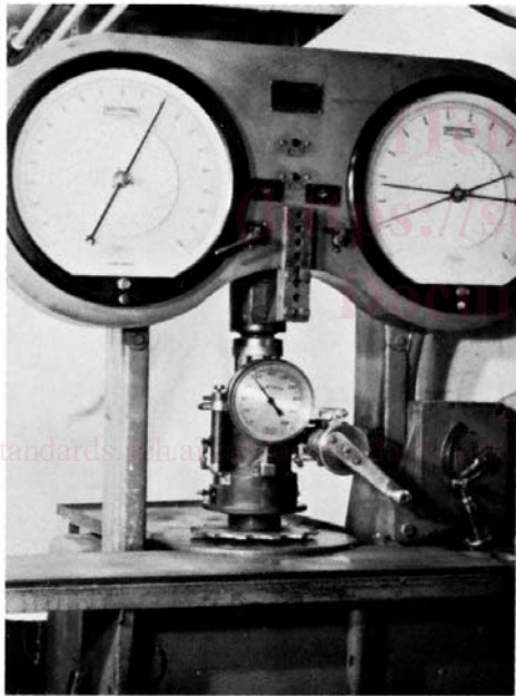
FIG. 3 Hveem Stabilometer Placed in the Testing Machine
