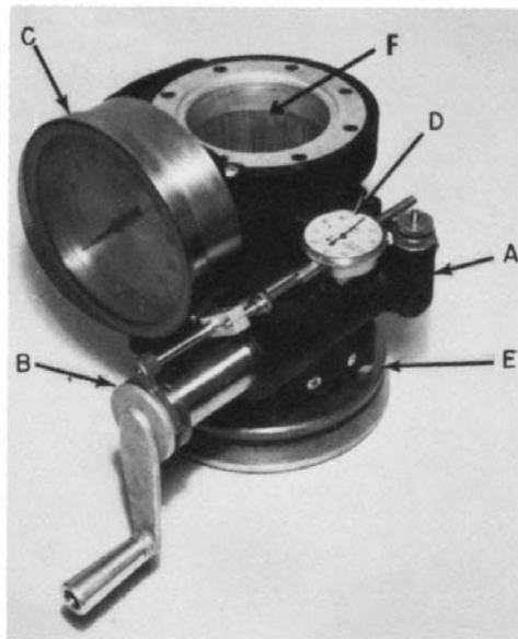
A—Air cell. B—Displacement pump. C—200-psi pressure gauge. D—Ames dial. E—Base adjustment nut. F—Bottom of upper tapered ring.
