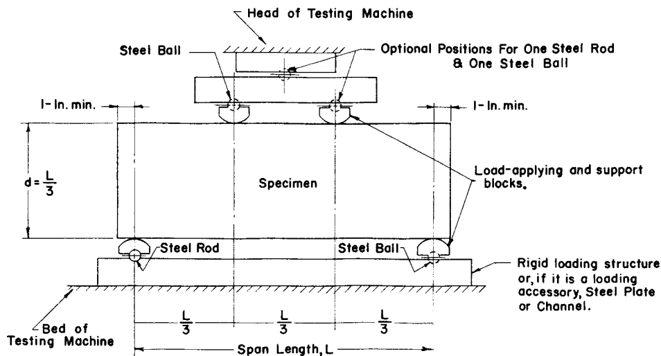
FIG. 1 Diagrammatic View of a Suitable Apparatus for Flexure Test of Refractory Mortar Joints, Four-Point Loading Method
