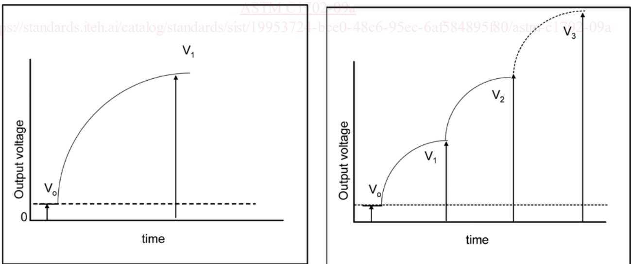
FIG. 2 (A) Schematic Steady-State Calibration Using A 2-Point Calibration Process And (B) Multi-Point Calibration Process
