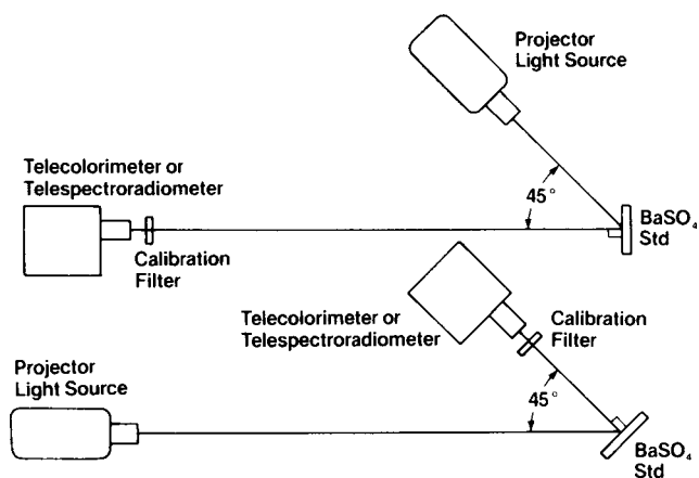
FIG. 1.2 Two Arrangements Suitable for Calibration of Telecolorimeter or Telespectroradiometer
