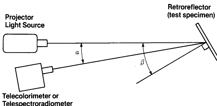
FIG. 2 1 Simplified Geometric Arrangement of Apparatus for Measurement of Chromaticity of Test Specimen
