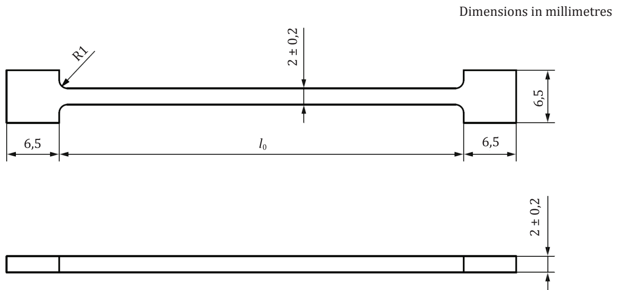
Figure 2 — Test piece
