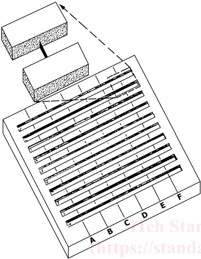
FIG. 1 H-Test Specimen
