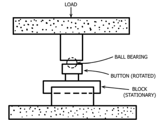
FIG. 2 Schematic Diagram of Galling Test Set-Up
