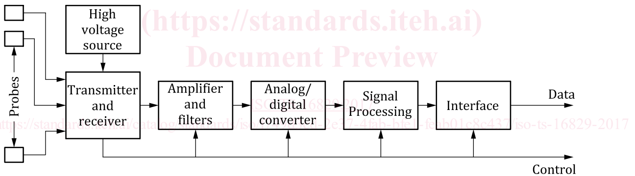
Figure 4 — Block diagram of the electronics of the ultrasonic sub-system
