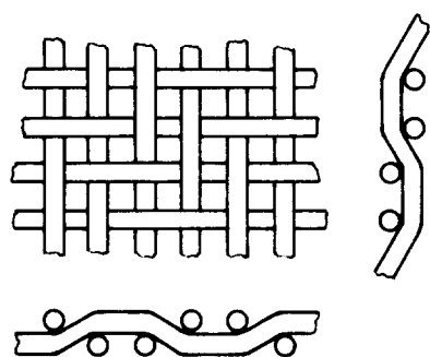
FIGURE 2 – Twilled weave
