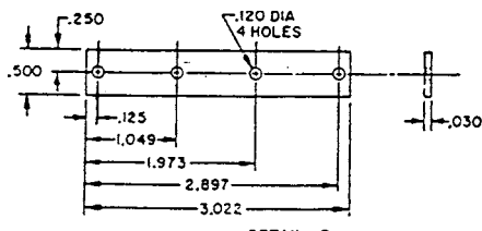
FIG. 7 Test Fixture Construction, Older Design (Fixture B)
