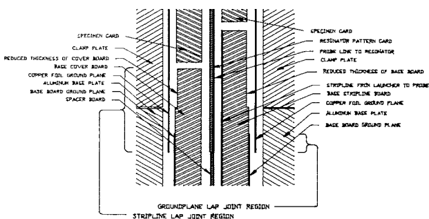
FIG. 3 Enlarged Exploded Side View Sectioned Through a Probe Line Showing a Lap Conductor Joint for Fixture A
