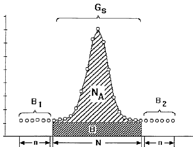
FIG. 1 Typical Spectral Peak With Parameters Used in the Peak Area Determination Indicated
