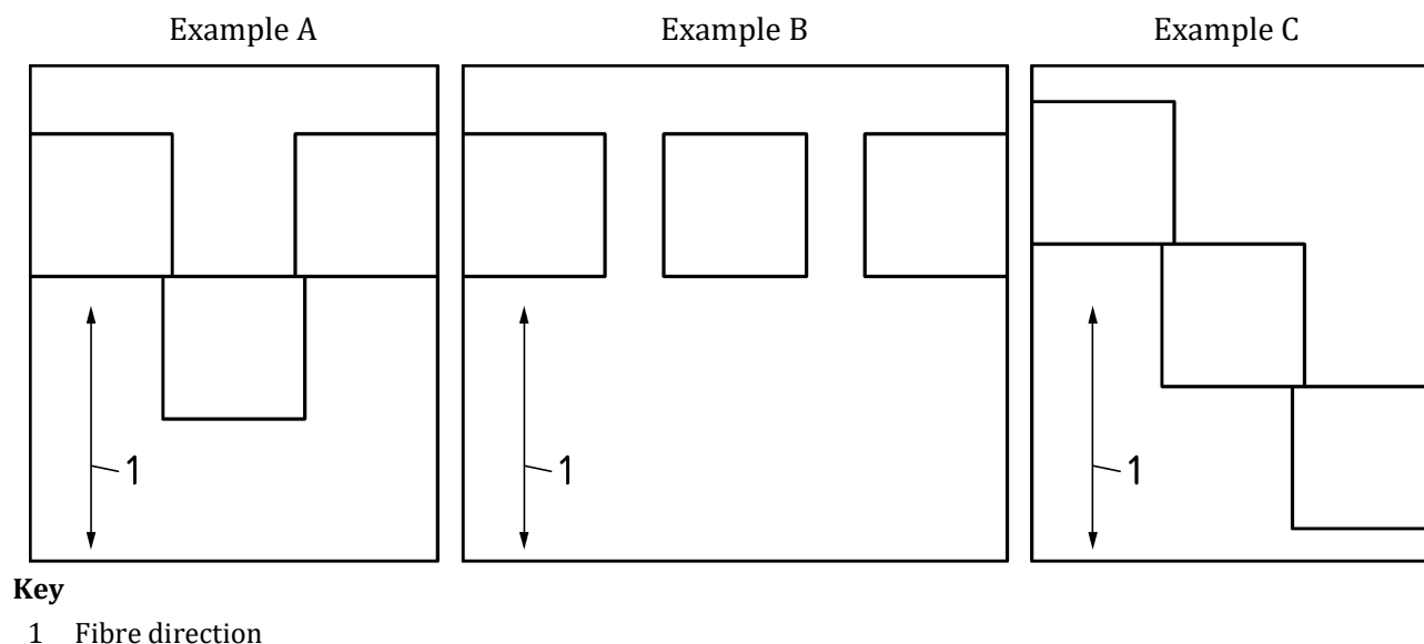
Figure 3 — Examples of possible positioning of specimens on carbon fibre unidirectional sheet or tape sample
