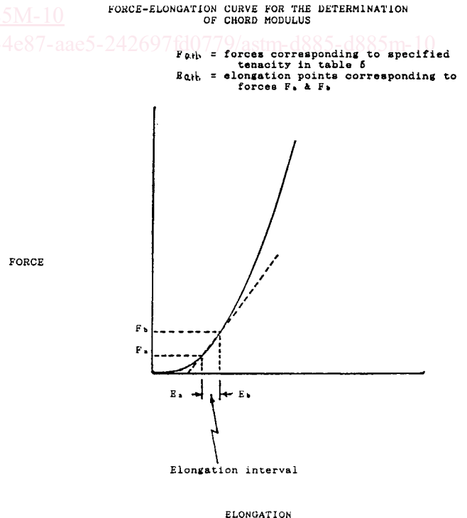
FIG. 3 Force-Elongation Curve for the Determination of Chord Modulus
