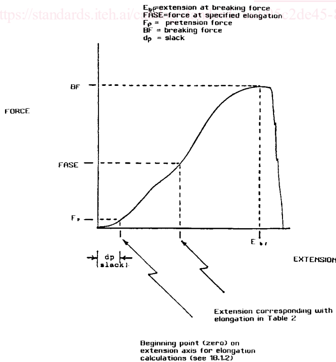
FIG. 1 Force-Extension Curve
