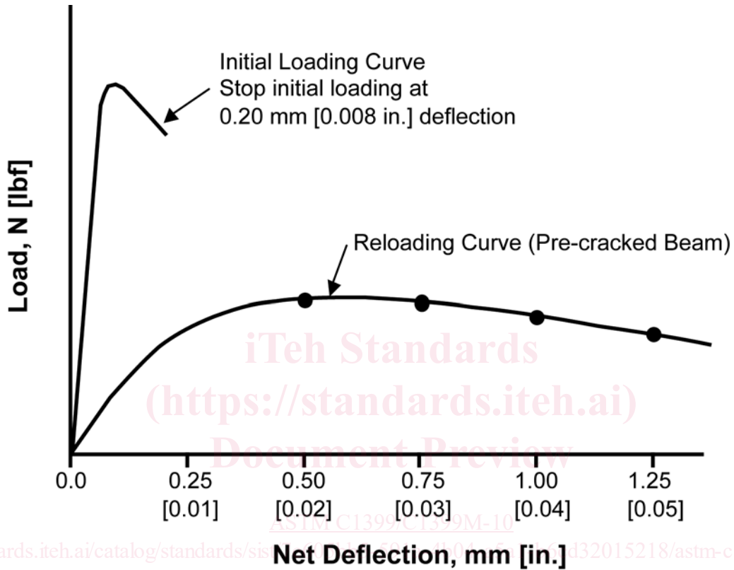
FIG. 2 Load-Deflection Curves
