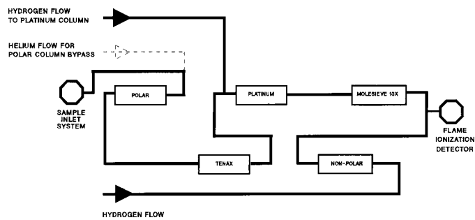
FIG. 11 Back Flush of the Polar Column
