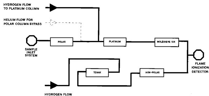
FIG. 11 Back Flush of the Polar Column
