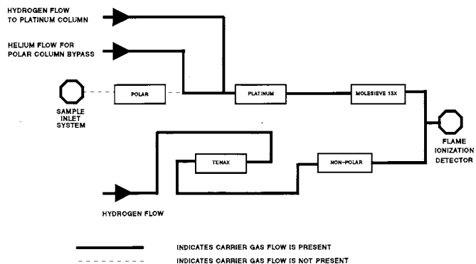
FIG. 6 End of the "B" Time
