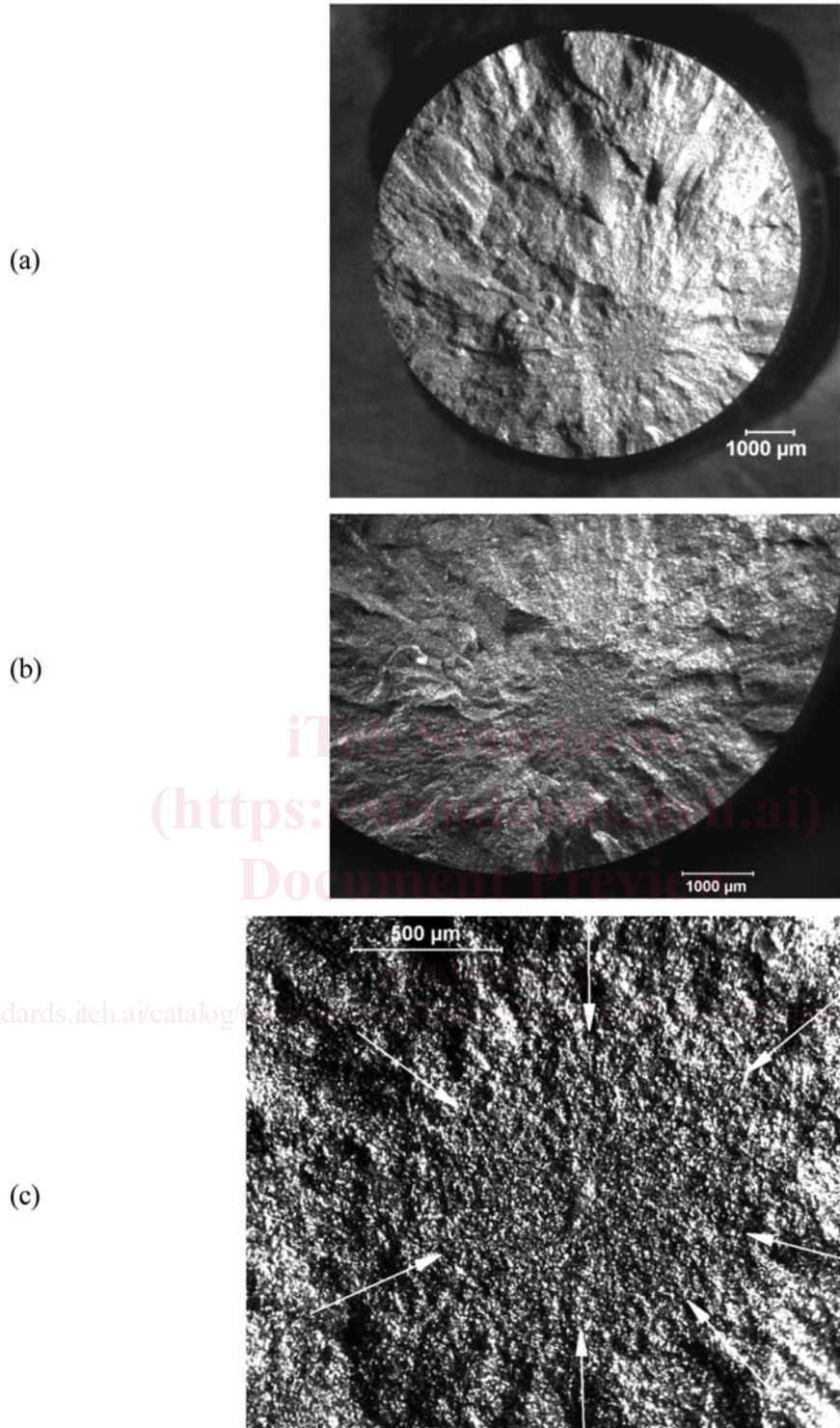
FIG. 3 Silicon Carbide Tension Strength Specimen (371 MPa) with a Mirror Centered on a Compositional Inhomogeneity Flaw.
