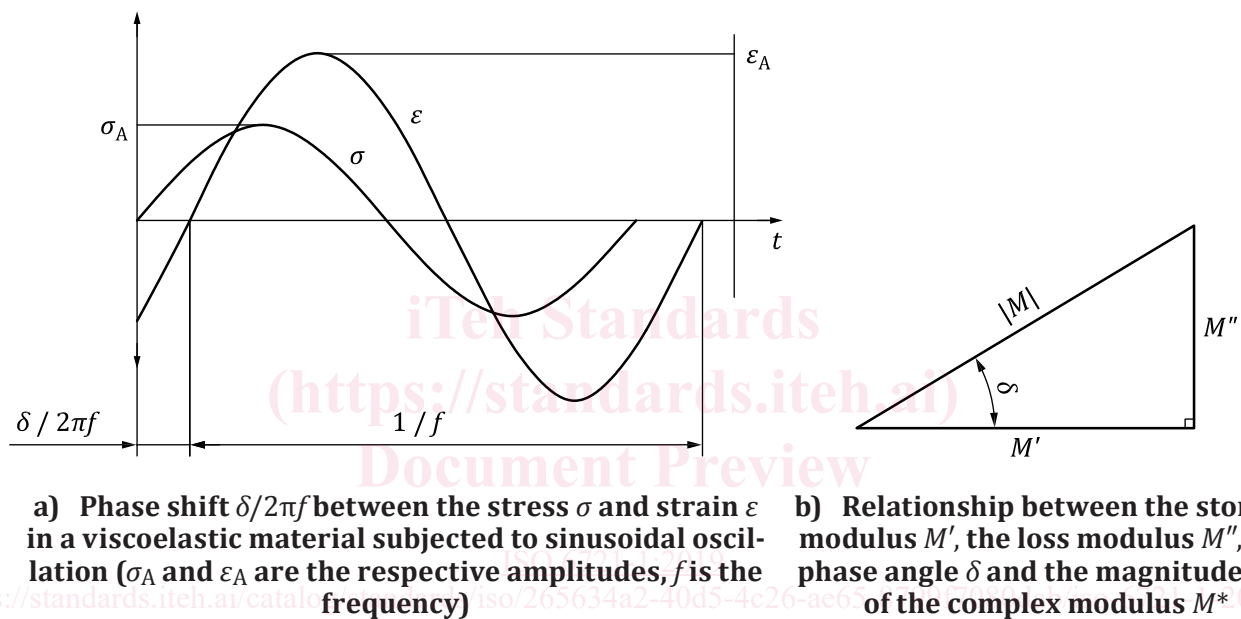
Figure 1 — Phase angle and complex modulus
