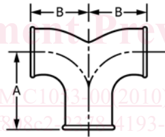
FIG. 12 Compact Single Sanitary T
