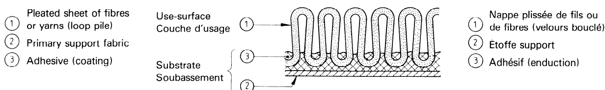
Figure 14 — Bonded-pile carpet (loop pile) (longitudinal section)
