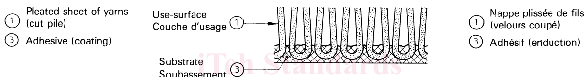
Figure 15 — Bonded-pile carpet (cut pile) (longitudinal section)
