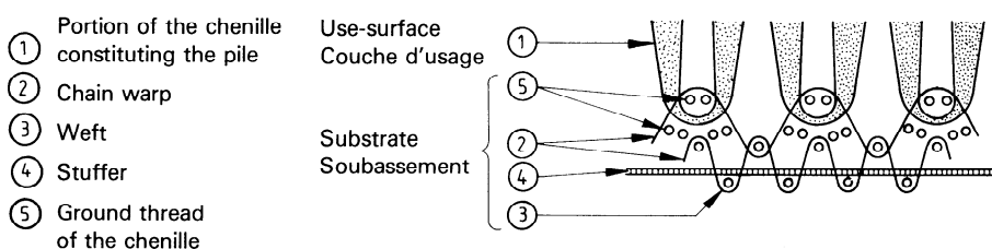
Figure 7 — Chenille Axminster carpet (warpways section)
