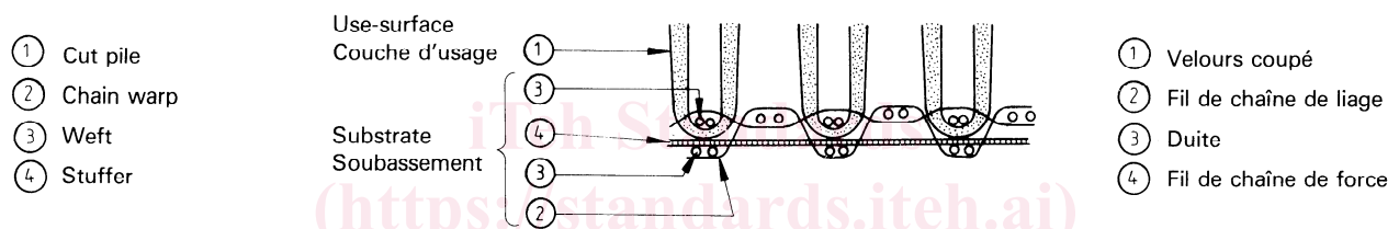
Figure 9 — Gripper Axminster carpet (warpways section)
