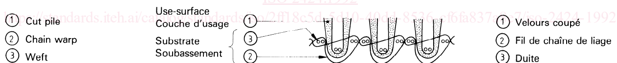
Figure 10 — Gripper Axminster carpet (Kardax construction)
