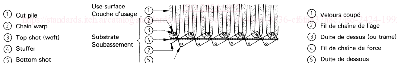
Figure 1 — Cut-pile, plain-woven carpet, two-shot (warps section)
