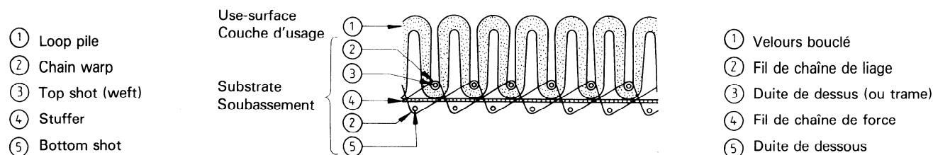
Figure 2 — Loop-pile, plain-woven carpet, two-shot (warps section)
