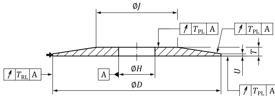
Figure 2 — Meule conique (Type 3)
