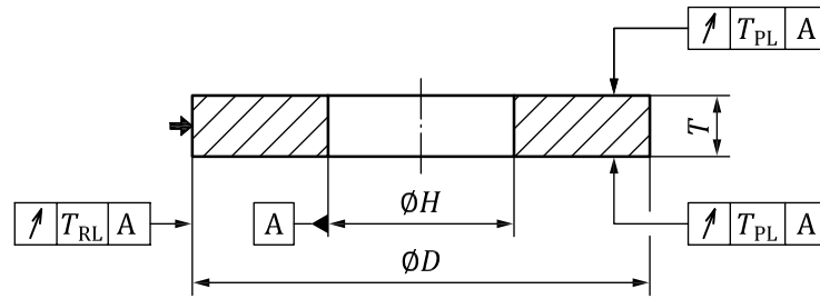
Figure 1 — Meule plate (Type 1)
