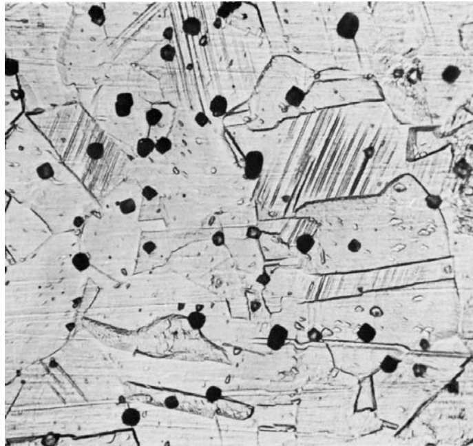
This or a greater concentration of end grain pits at 500× (using standard etching conditions) indicates that the specimen must be tested when screening is for nitric acid test.
