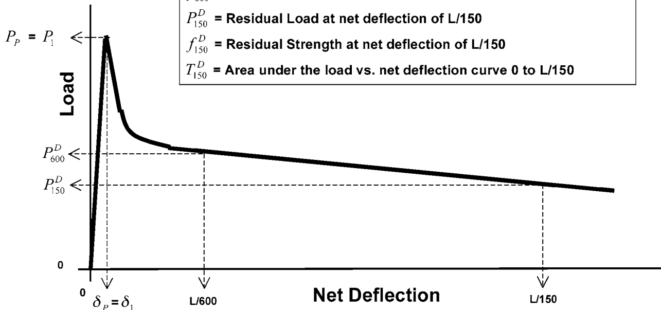
FIG. 3 Example of Parameter Calculations for First-Peak Load Equal to Peak Load (Not to Scale)
