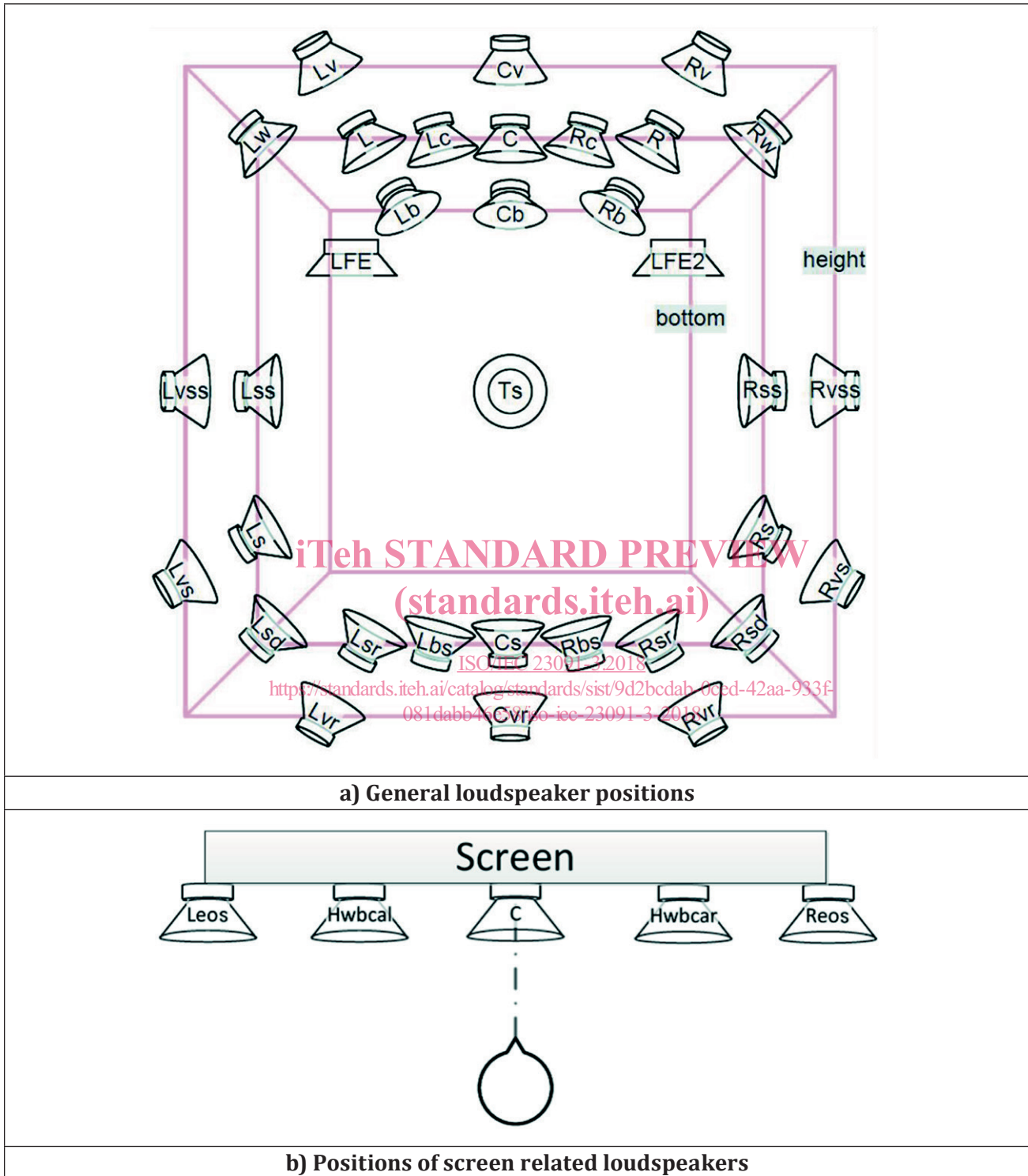
Figure 2 — Loudspeaker positions
