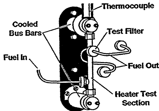
FIG. 1 Standard Heater Section, Essential to All JFTOT D3241 Test Instruments
