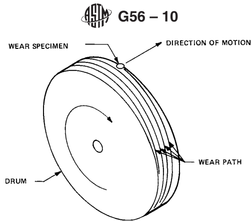
FIG. 2 Test Motion
