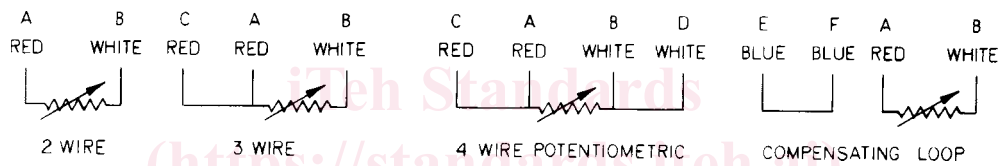
FIG. 2 Connection Configurations
