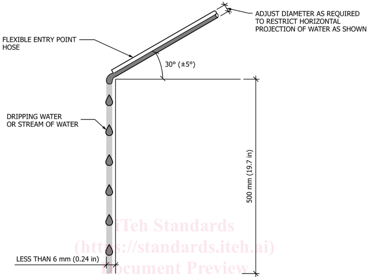
FIG. 3 Entry Point Hose
