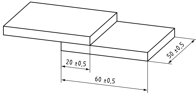
Figure 3 — Shear test specimen
