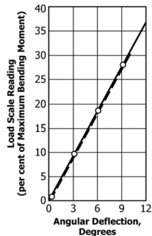
FIG. 2 Ideal Curve
