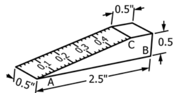
NOTE 1—SI Equivalents (Dimensions are in inchs.)
