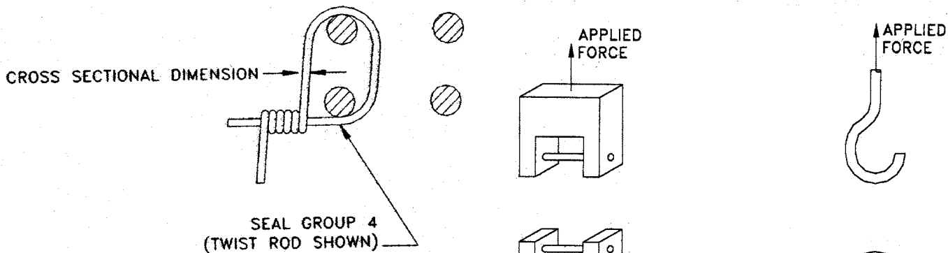
FIG. 3 Schematic Drawings of Pull (Tensile) Test Fixture Requirements for Group 4
