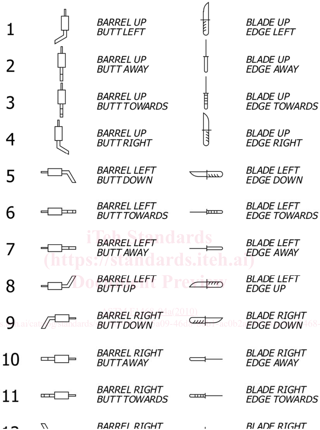
FIG. 1 Test Object Orientation
